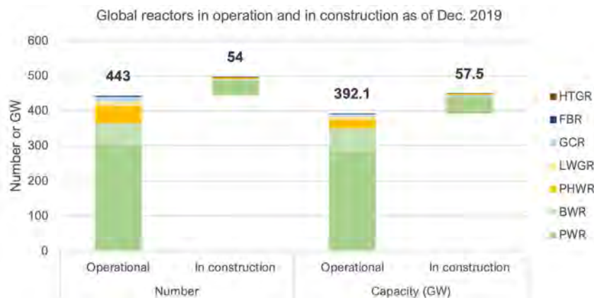
Figure 33 Snapshot of global nuclear power reactors, operational and in construction, as of December 2019
