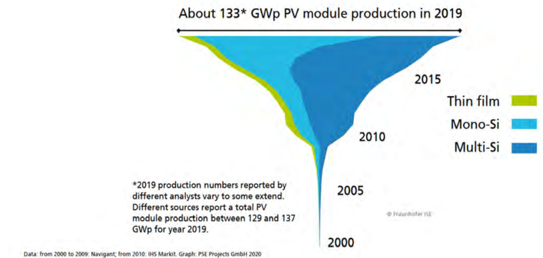
Figure 18 Global photovoltaic module production by main technology
