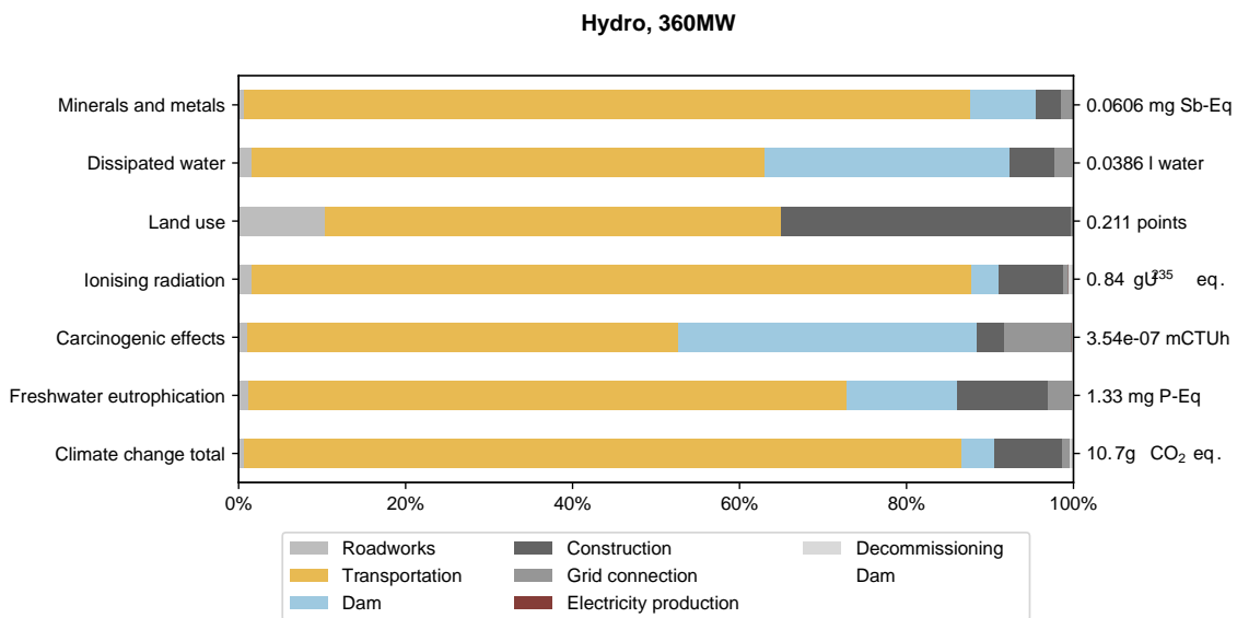
Figure 32 Life cycle impacts from 1 kWh of hydropower production, based on a 360-MW plant design, Europe, 2020
