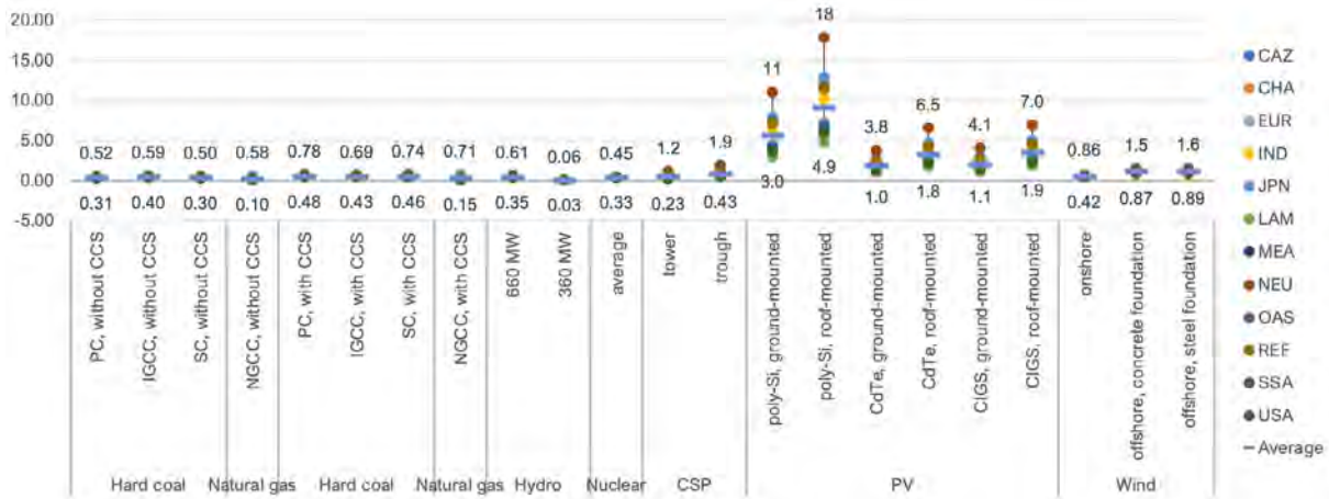
Figure 45 Lifecycle mineral and metal requirement, in g Sb eq. per MWh, regional variation, 2020
